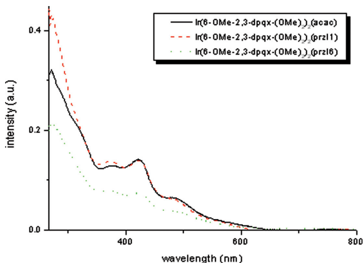
FIGURE 2 UV-Vis absorption spectra of the iridium complexes in a 10^{-5} M \text{CH}_2\text{Cl}_2 solution.
