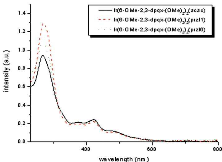
FIGURE 3 UV-Vis absorption spectra of PMMA film containing the Ir complexes.
