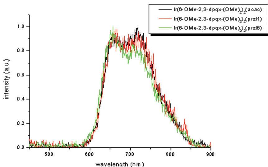
FIGURE 5 PL spectra of PMMA film containing the Ir complexes.
