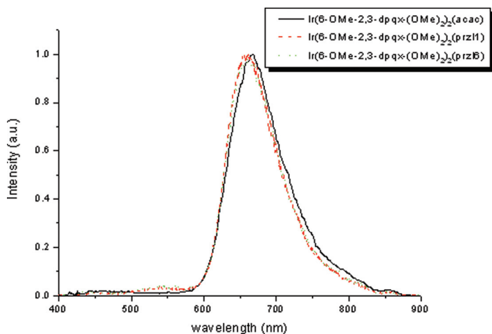
FIGURE 4 PL spectra of the iridium complexes in a 10^{-5} M \text{CH}_2\text{Cl}_2 solution.
