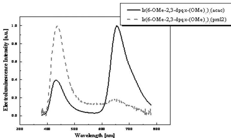
FIGURE 6 EL spectra of the Ir complexes.
